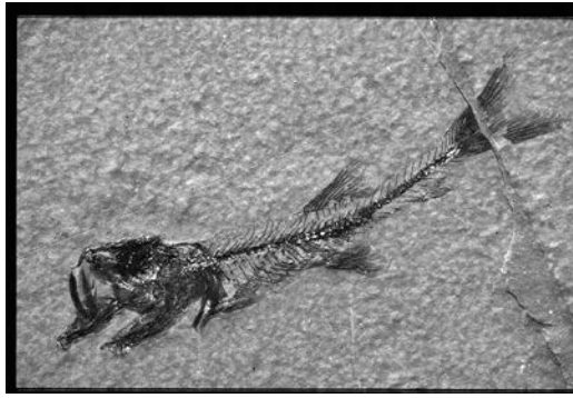
"Ascalabos" sp.
